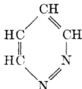
Pyridazine
