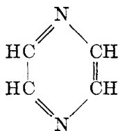
Pyrazine
